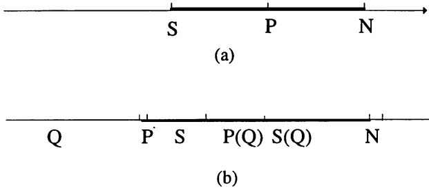
Figure 2: Equilibrium in one-dimensional legislative choices
